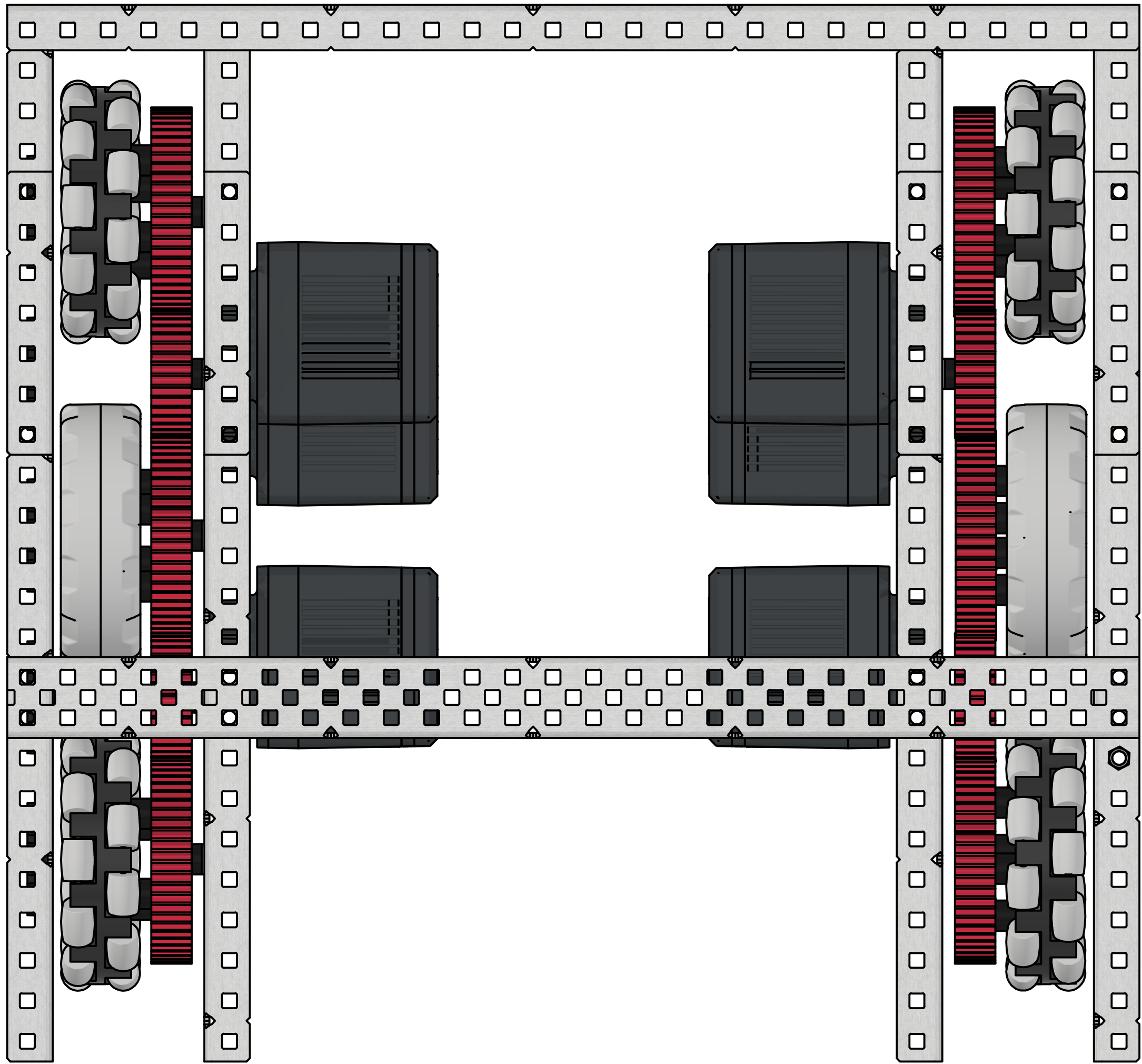
Top View
